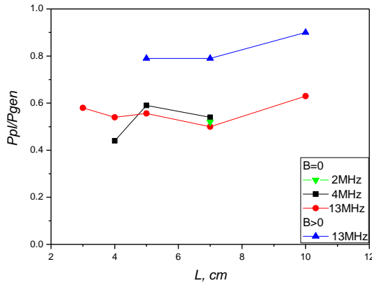
Figure 10. Efficiency of the radio-frequency power coupling to plasma vs the length of the discharge chamber. Xenon, 4 sccm, P_{gen} = 110W .
